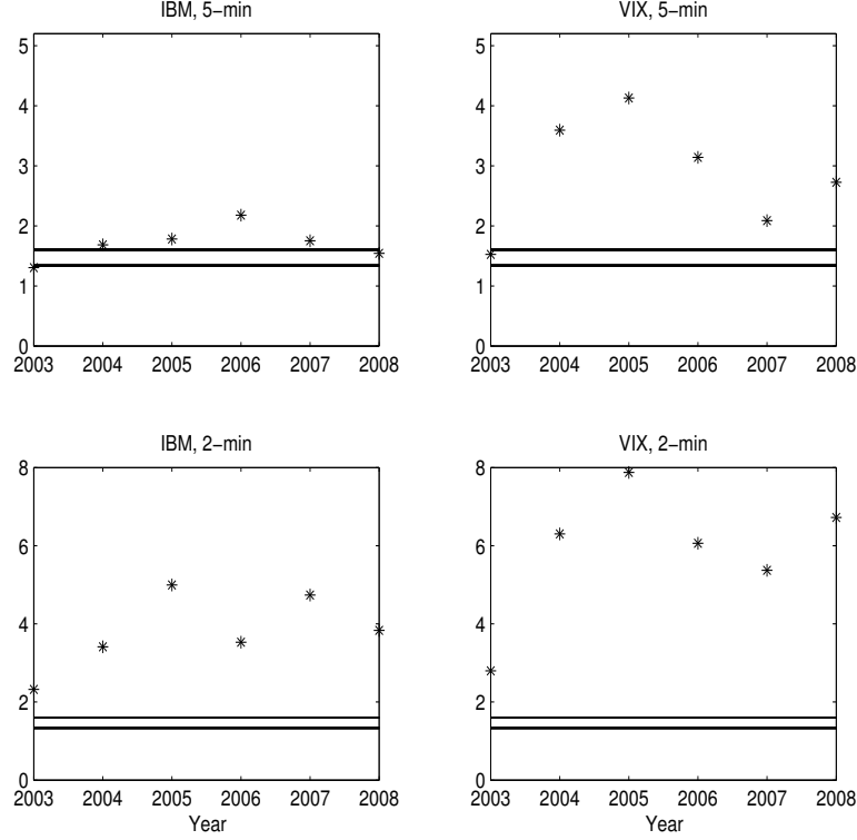
FIG 1. Kolmogorov-Smirnov tests for local Gaussianity. The * corresponds to the value of the test \sup_{\tau \in \mathcal{A}} \sqrt{N^n}(\alpha, \varpi) |\widehat{F}_n(\tau) - F(\tau)| and the solid lines are the critical values q_n(\alpha, \mathcal{A}) for \alpha = 5\% and \alpha = 1\% .
